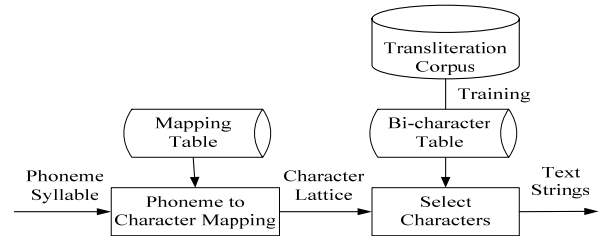
Figure 3. Flow Chart of Phoneme-Character Conversion
