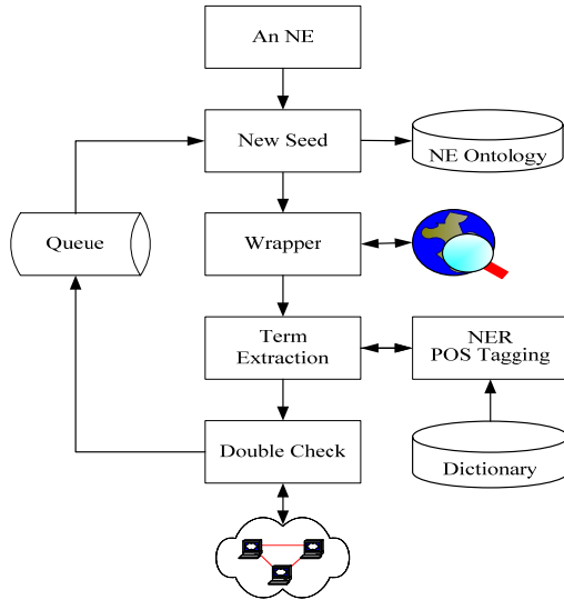
Figure 1. Flow of Named Entity Ontology Generation
