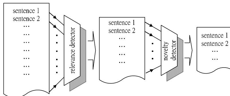
Figure 1: Architecture of Our Novelty System
