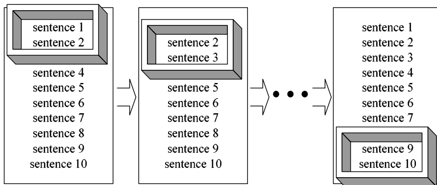
Figure 3: A Sliding Window (window size = 2)
